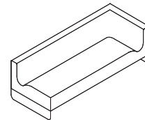
Sofa w/ right arm CAN25RIT L 211cm D 90cm H 60cm L 83" D 35½" H 23½"
